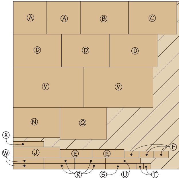
60" x 60" - 1/2" PLYWOOD
