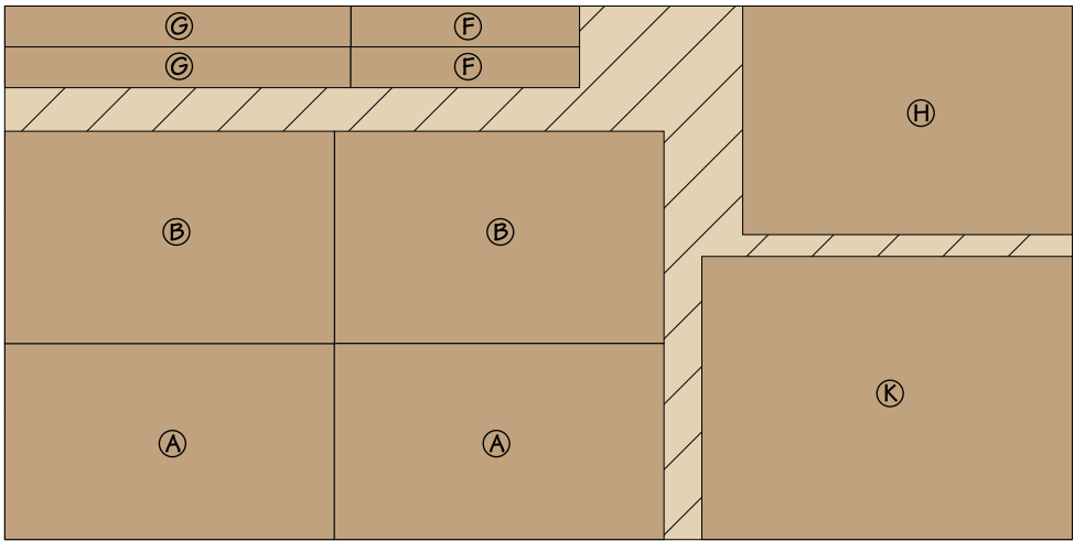
49" x 97" - 3/4" MDF
