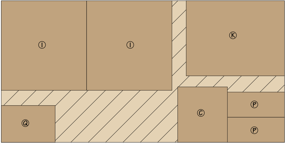
49" x 97" - 3/4" MDF
