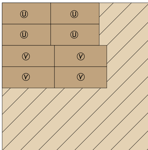
48" x 48" - 1/2" PLYWOOD
