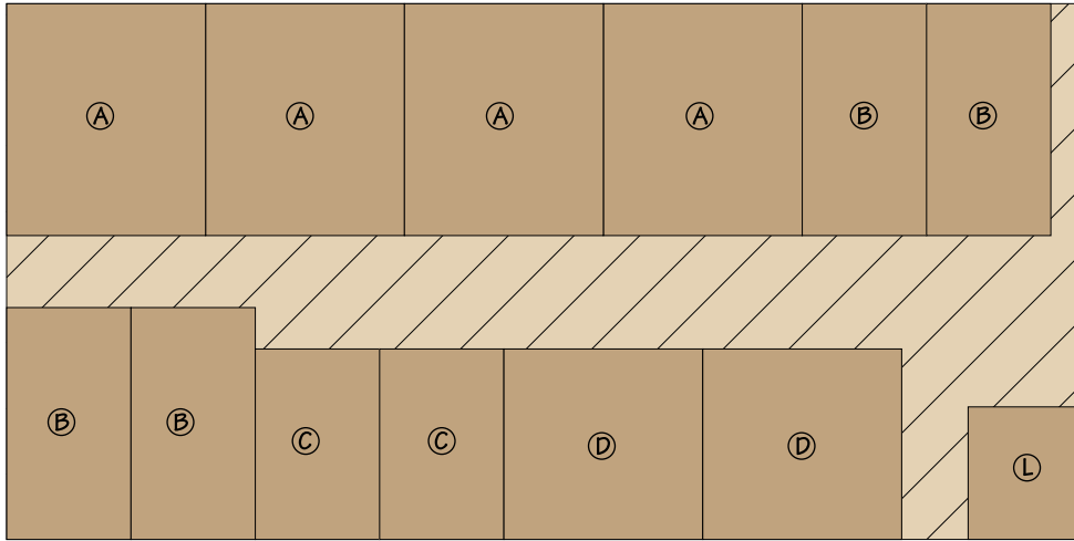
49" x 97" - 3/4" MDF
