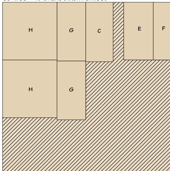
60" x 60" - ¾" BALTIC BIRCH PLYWOOD
