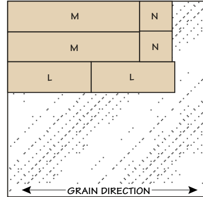
48" x 48" - 3/4" PLYWOOD
