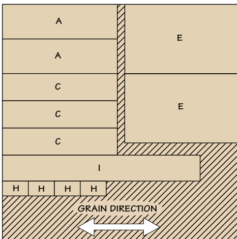
48" x 48" - 3/4" PLYWOOD
