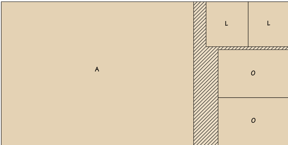
48" x 96" - 3/4" PLYWOOD
