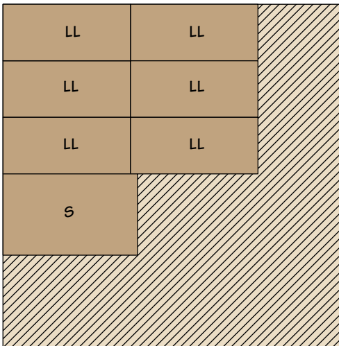
48" x 48" - 1/4" HARDBOARD
