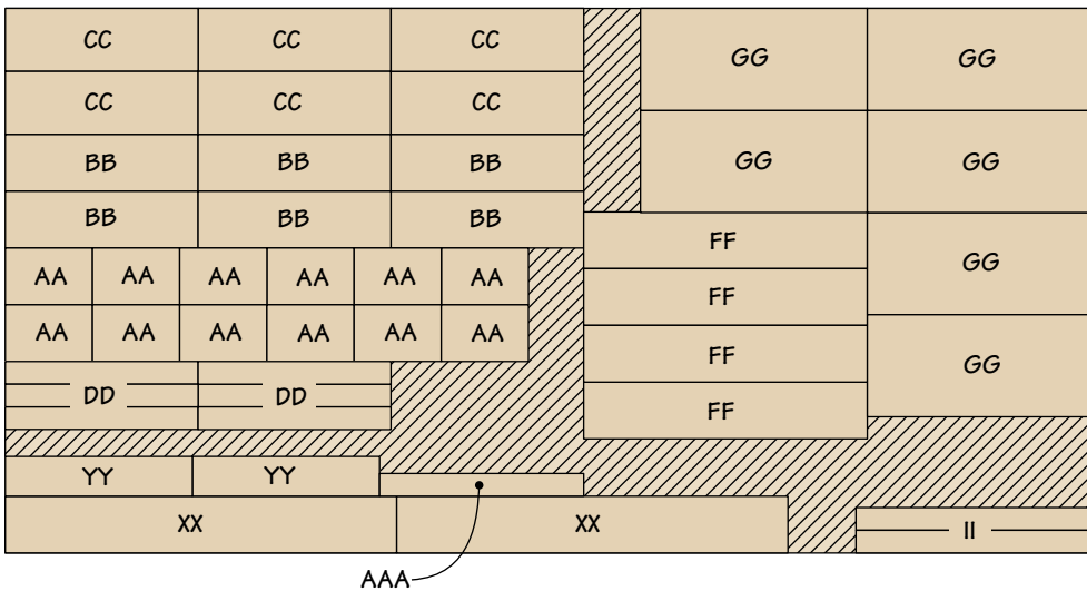
48" x 96" - 3/4" PLYWOOD
