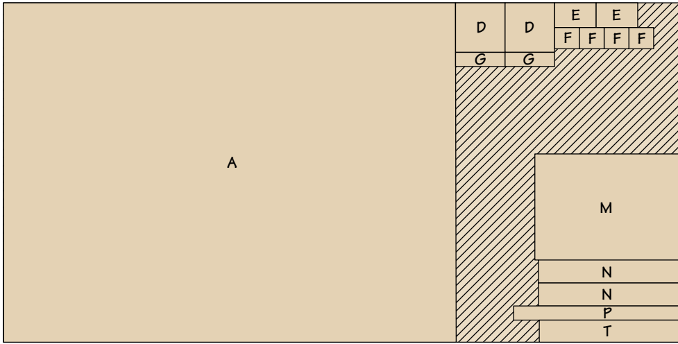
48" x 96" - 3/4" PLYWOOD
