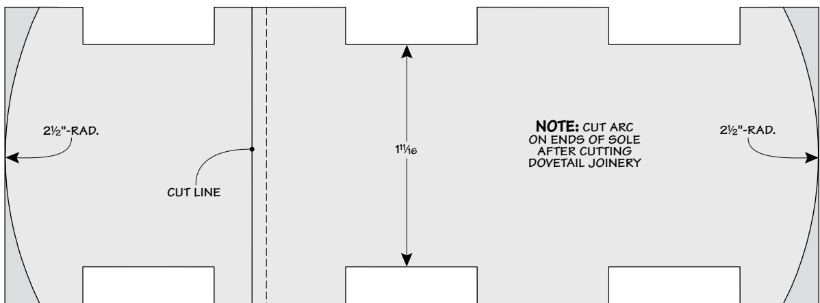
TOP VIEW (STEEL SOLE)
