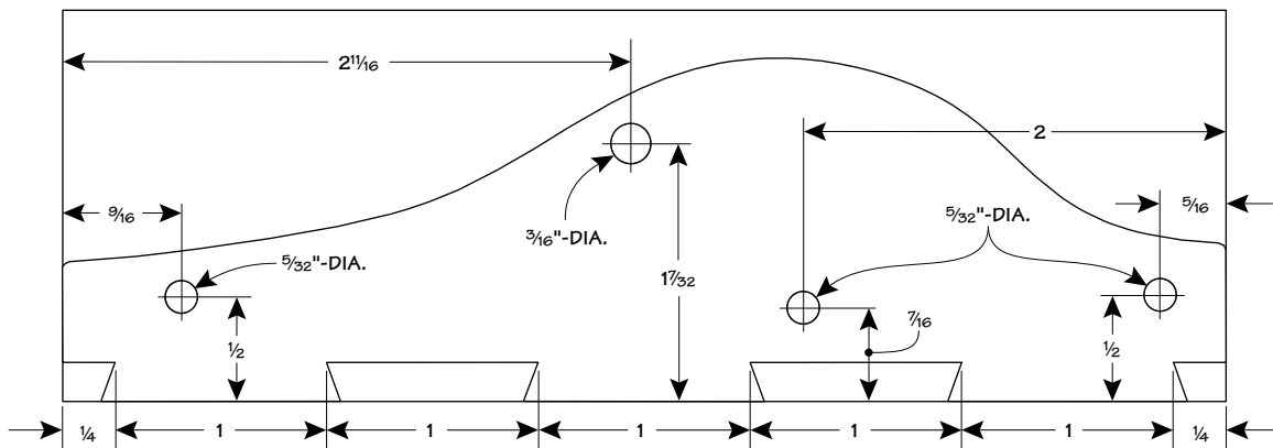
SIDE VIEW (BRASS SIDE)
